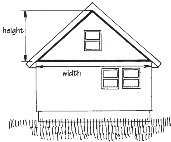
Figure 10. Gable areas
