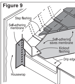
Figure 9, Kickout Flashing ‡ To prevent water from dumping behind the siding and the end of the roof intersection, install a "kickout" of sufficient length and angle to direct the water running down the roof away from the siding.
