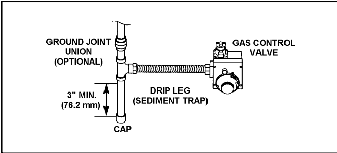
FIGURE 12. GAS PIPING WITH FLEXIBLE CONNECTOR.
