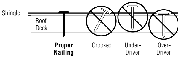
Figure 12-2: Proper and improper nailing.
