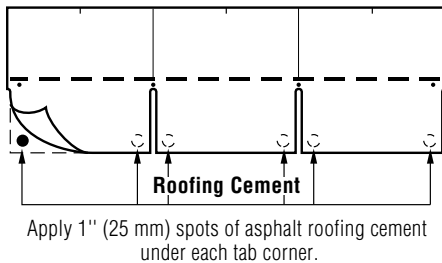
Figure 12-4: Use four nails and six spots of asphalt cement on steep slopes.
